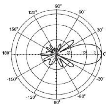
V-Plane Co-polarization Pattern
