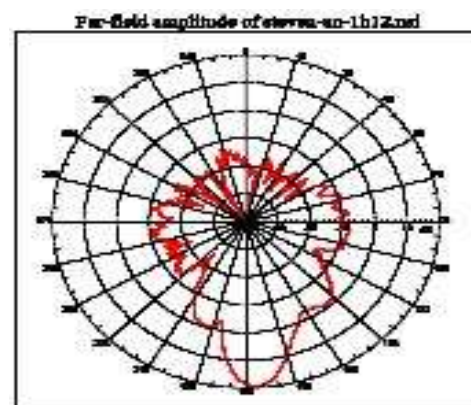
Horizontal-Plane Co-polarization
